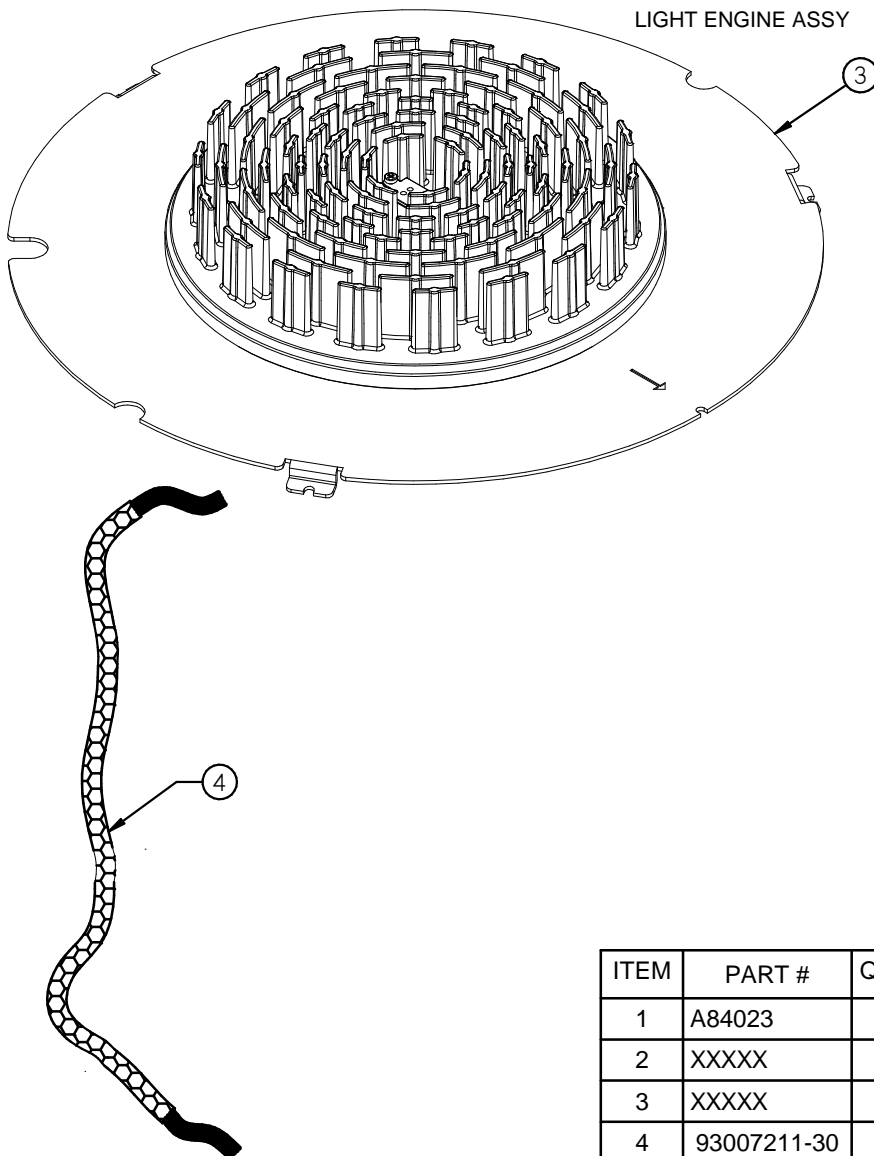
LIGHT ENGINE ASSY
