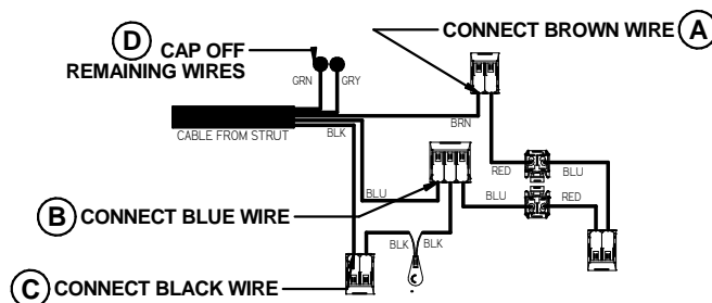
500 & 700 mA WIRING DIAGRAM
