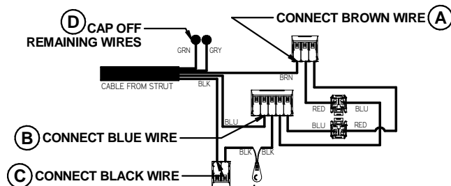
225, 335 & 345mA WIRING DIAGRAM
